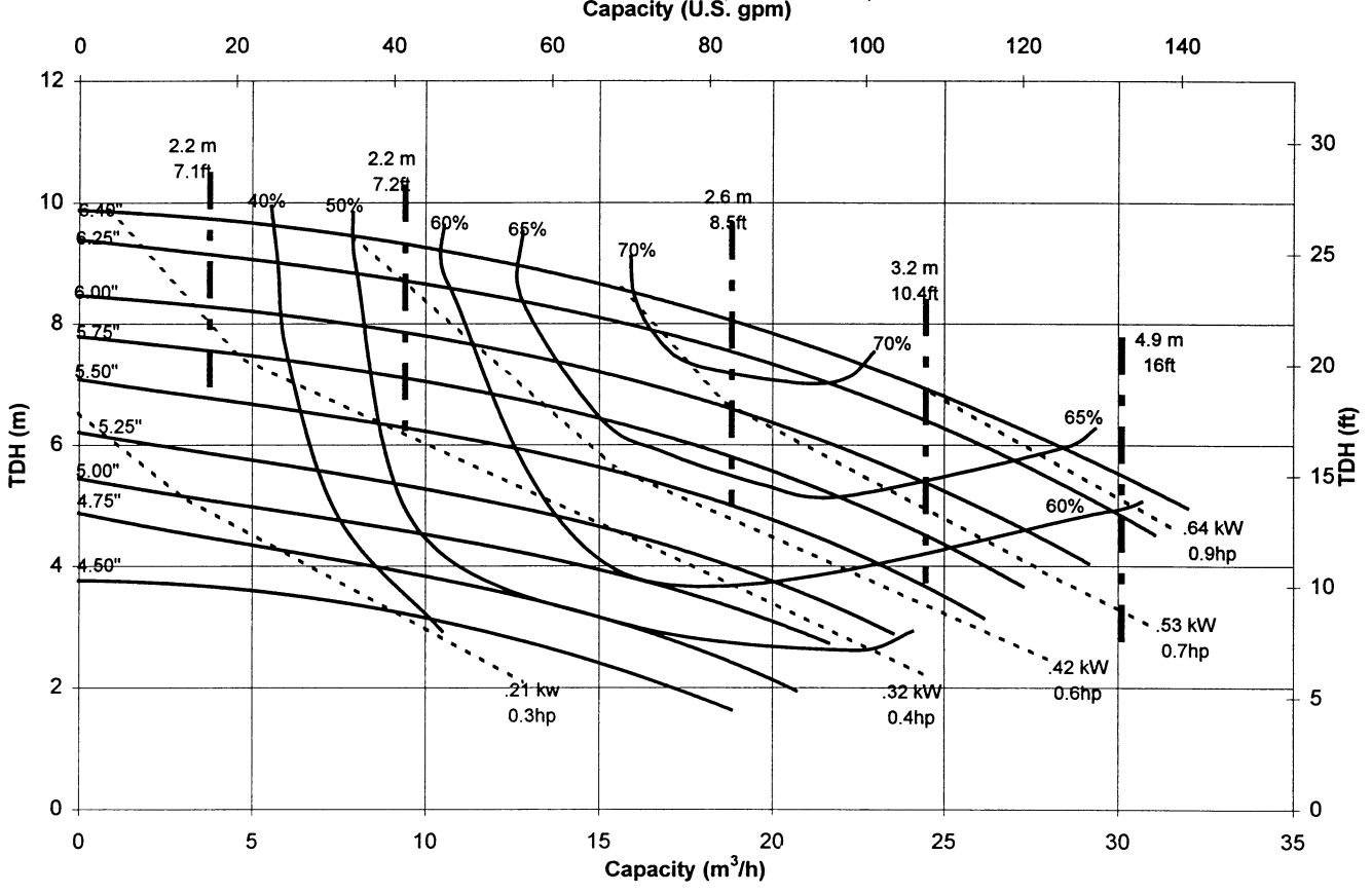
KV326 Performance Curve, 1450 RPM, S.G. 1.00
