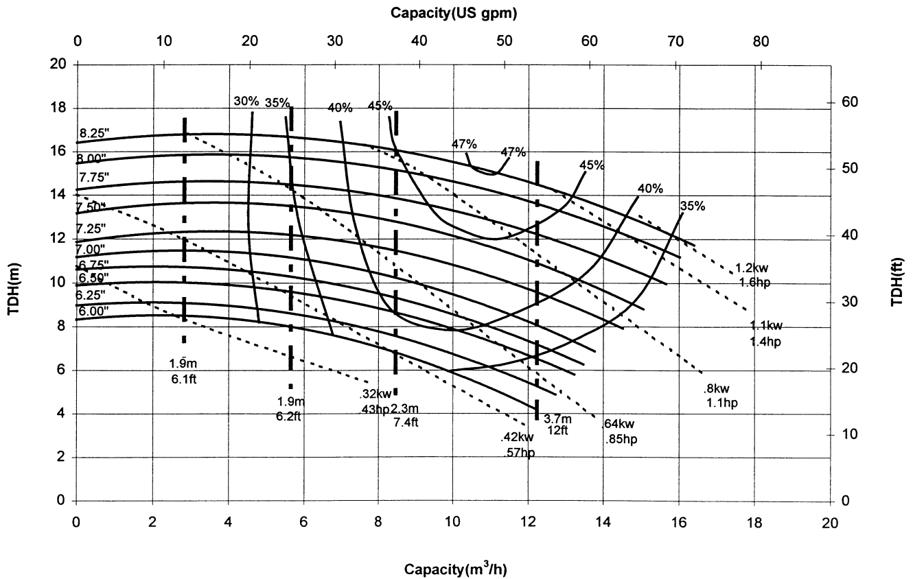
KV2158 Performance Curve, 1450 rpm, S.G. 1.00
