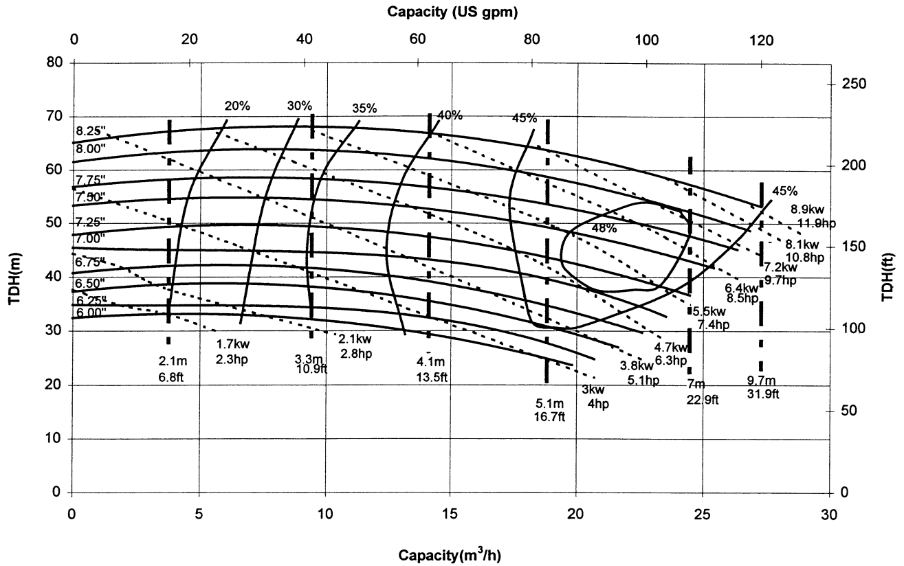
KV2158 Performance Curve, 1450 rpm, S.G. 1.00
