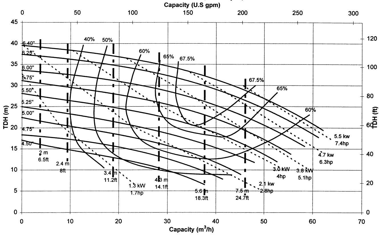
KV326 Performance curve, 2900 rpm, S.G. 1.00
