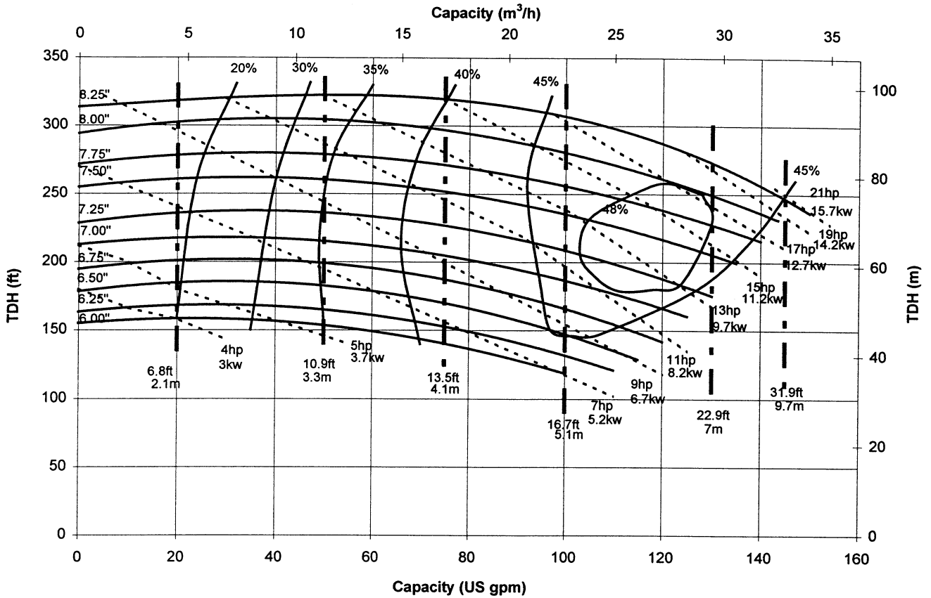
KV2158 Performance Curve, 1750 rpm, S.G. 1.00
