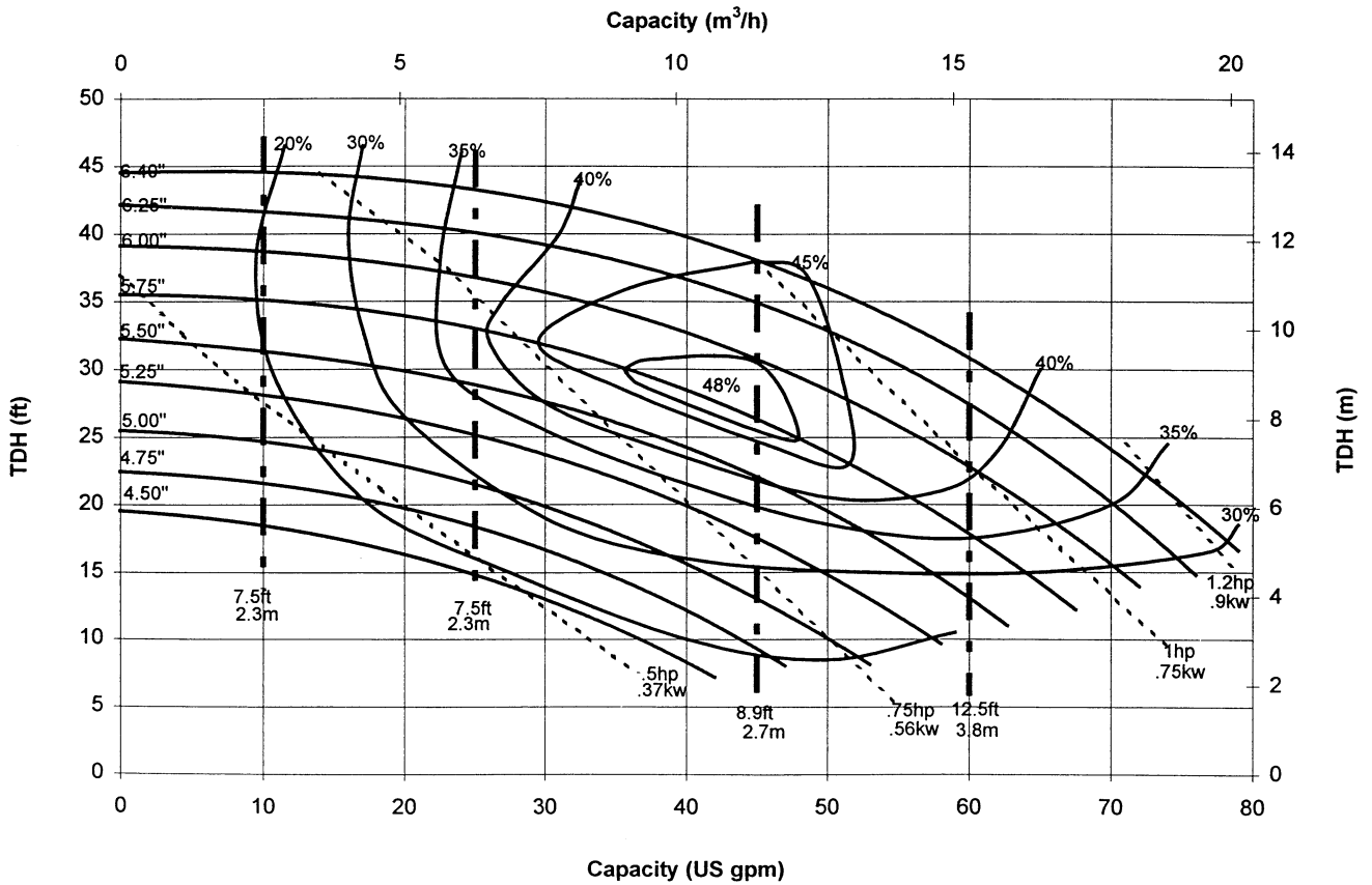
KV2156 Performance Curve, 1750 rpm, S.G. 1.00
